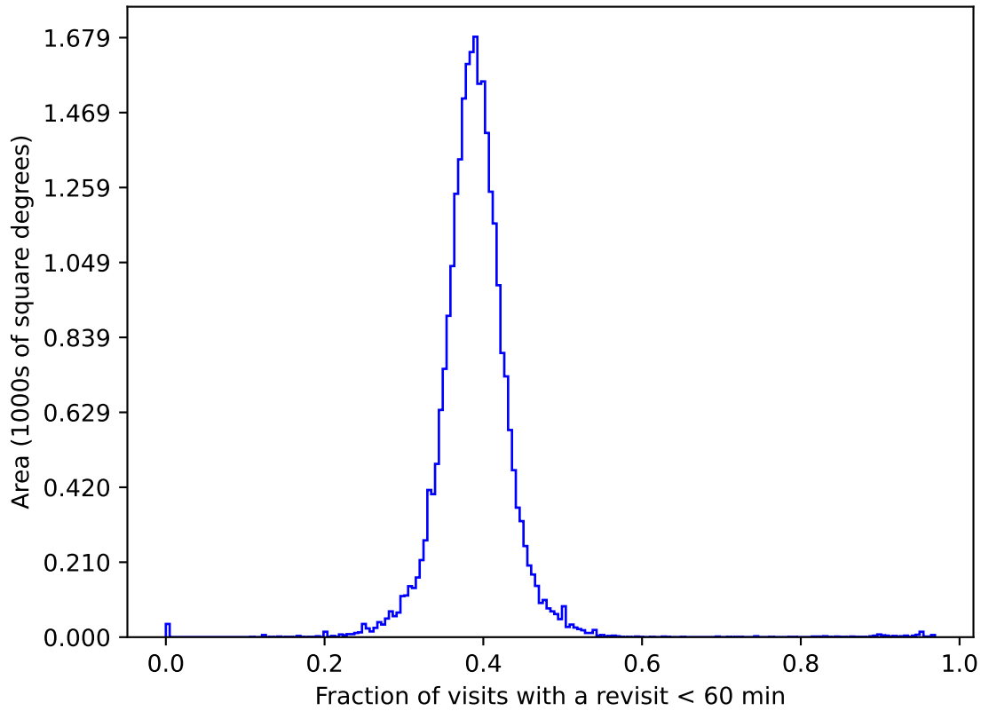
weather_cloudso20v3.4_10yrs gri All sky: Fraction of visits with a revisit < 60 min
