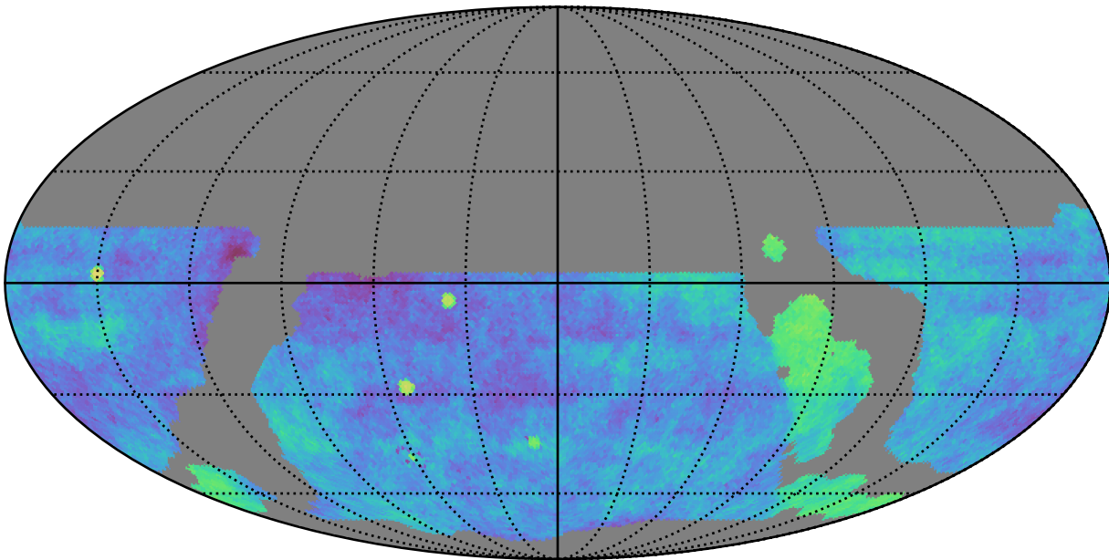
weather_cloudso20v3.4_10yrs gri WFD: Fraction of visits in pairs (20-90 min)
