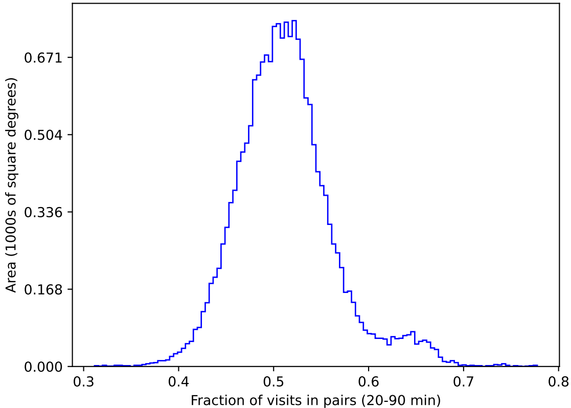
weather_cloudso20v3.4_10yrs gri WFD: Fraction of visits in pairs (20-90 min)
