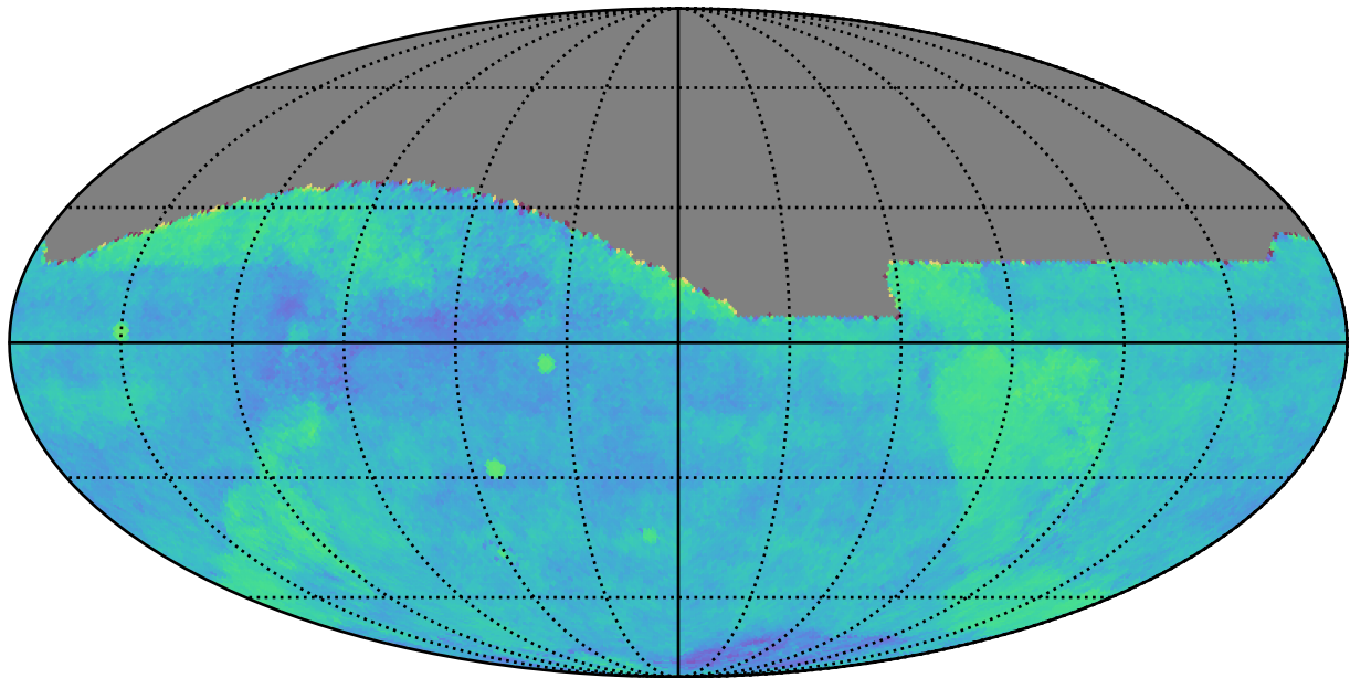
weather_cloudso20v3.4_10yrs gri All sky: Fraction of visits in pairs (20-90 min)
