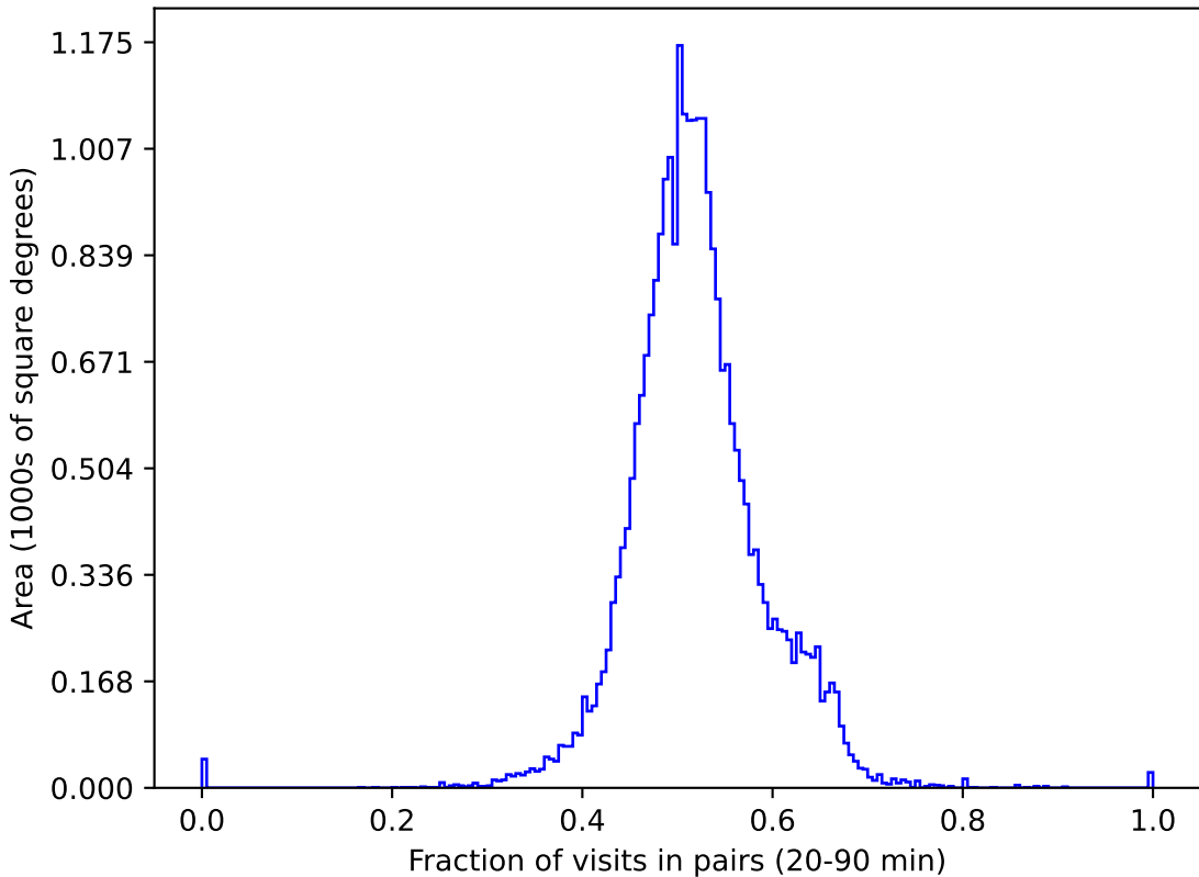
weather_cloudso20v3.4_10yrs gri All sky: Fraction of visits in pairs (20-90 min)
