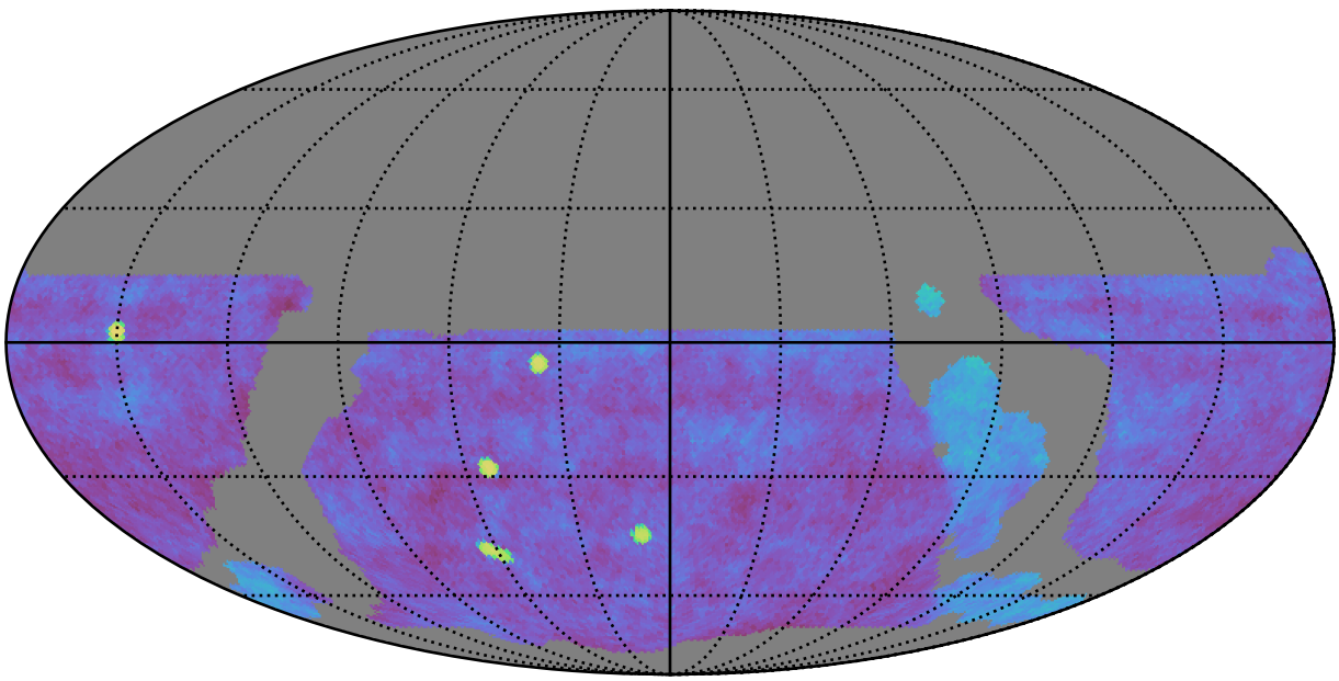
weather_cloudso20v3.4_10yrs gri WFD: Fraction of visits in pairs (10-60 min)
