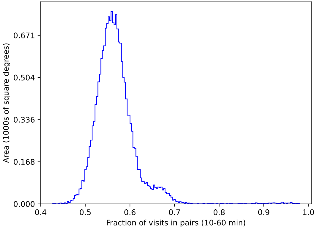
weather_cloudso20v3.4_10yrs gri WFD: Fraction of visits in pairs (10-60 min)
