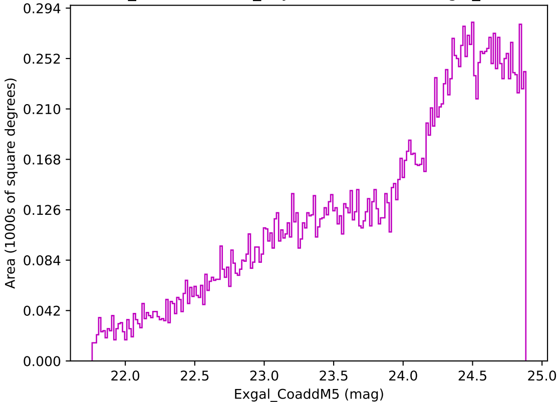
weather_cloudso20v3.4_10yrs Yr 3-4 z band: Exgal_CoaddM5
