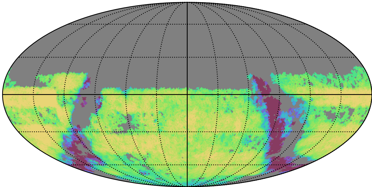
weather_cloudso20v3.4_10yrs Yr 3-4 u band: Exgal_CoaddM5
