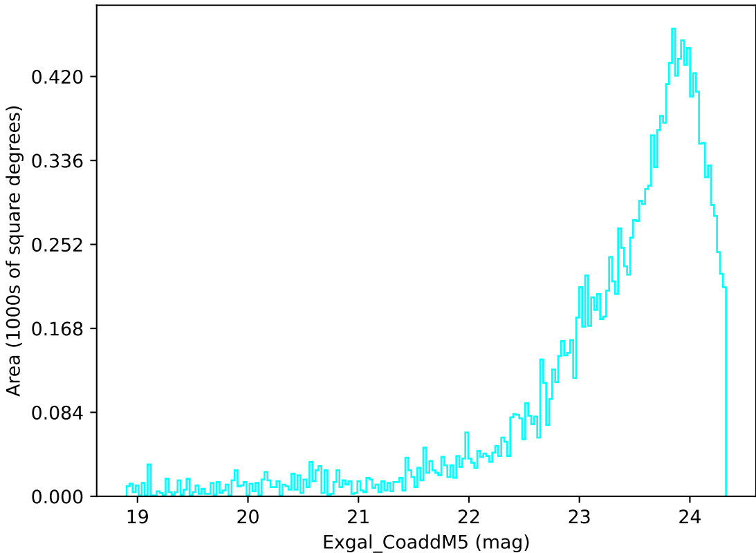
weather_cloudso20v3.4_10yrs Yr 3-4 u band: Exgal_CoaddM5
