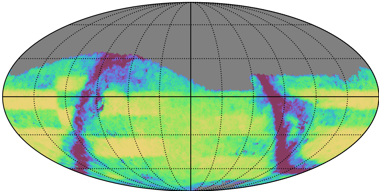
weather_cloudso20v3.4_10yrs Yr 3-4 r band: Exgal_CoaddM5
