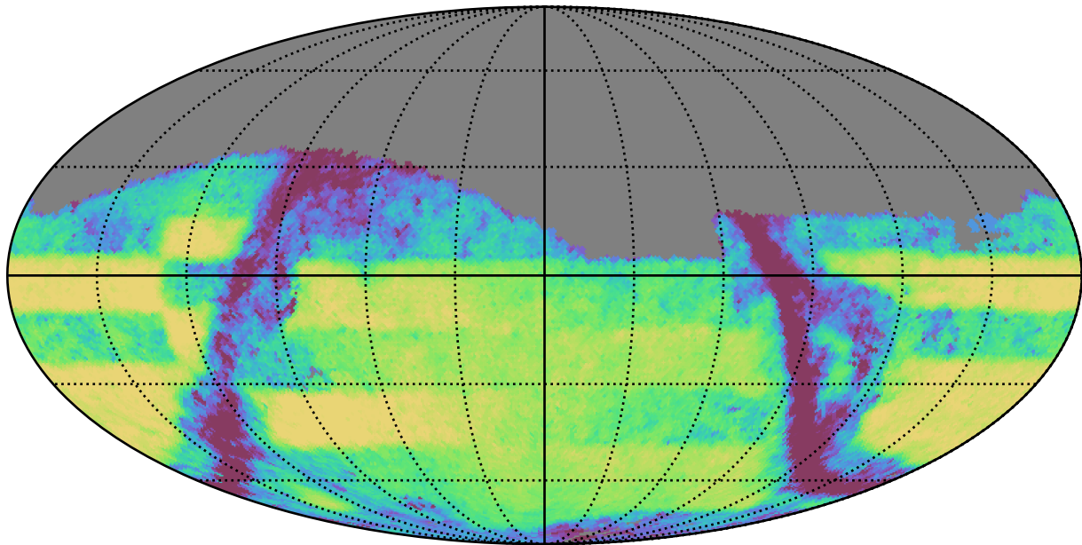
weather_cloudso20v3.4_10yrs Yr 3-4 i band: Exgal_CoaddM5
