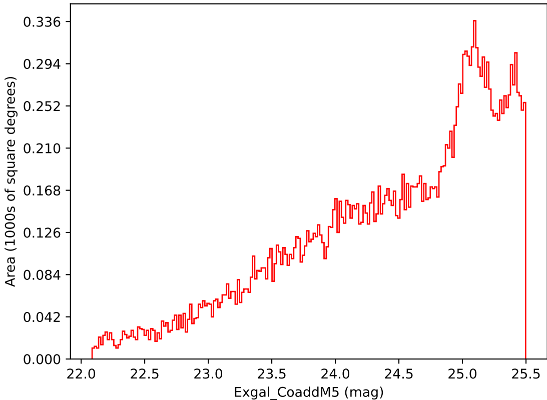
weather_cloudso20v3.4_10yrs Yr 3-4 i band: Exgal_CoaddM5
