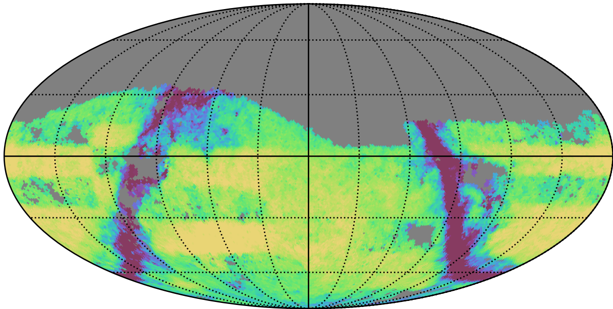
weather_cloudso20v3.4_10yrs Yr 3-4 g band: Exgal_CoaddM5
