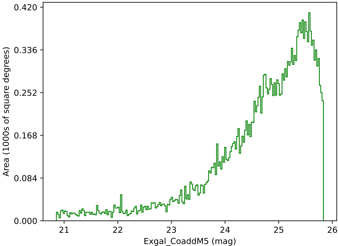
weather_cloudso20v3.4_10yrs Yr 3-4 g band: Exgal_CoaddM5
