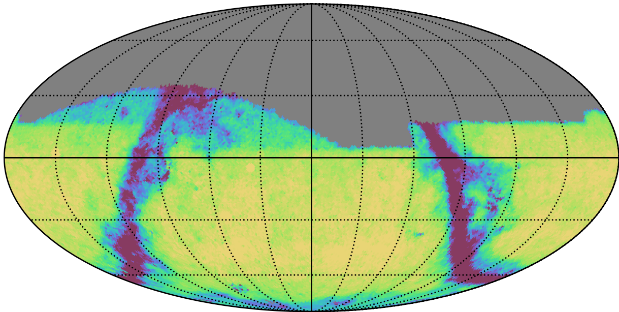
weather_cloudso20v3.4_10yrs Yr 1 r band: Exgal_CoaddM5
