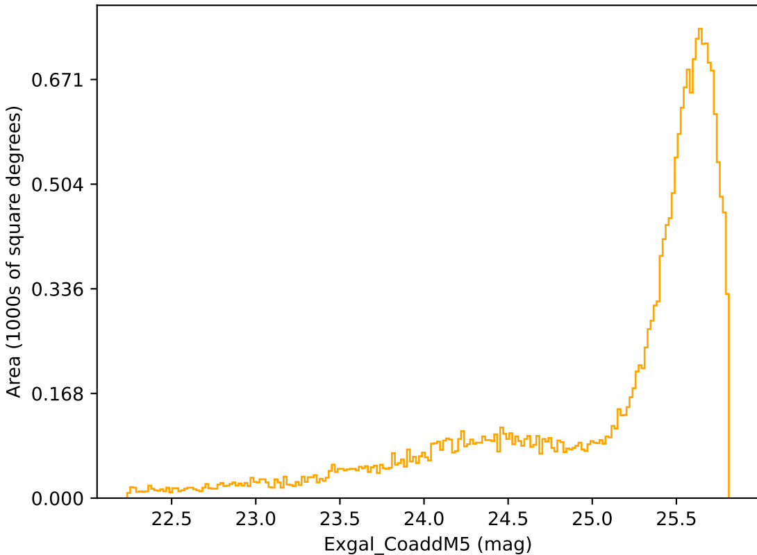
weather_cloudso20v3.4_10yrs Yr 1 r band: Exgal_CoaddM5
