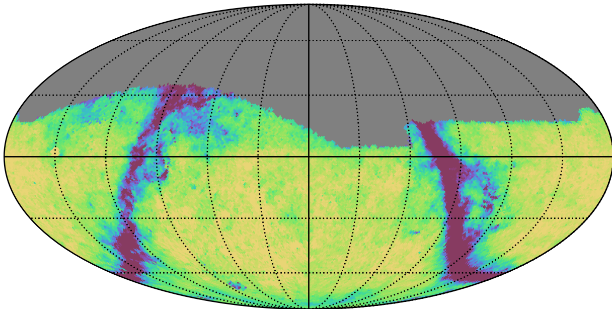
weather_cloudso20v3.4_10yrs Yr 1 g band: Exgal_CoaddM5
