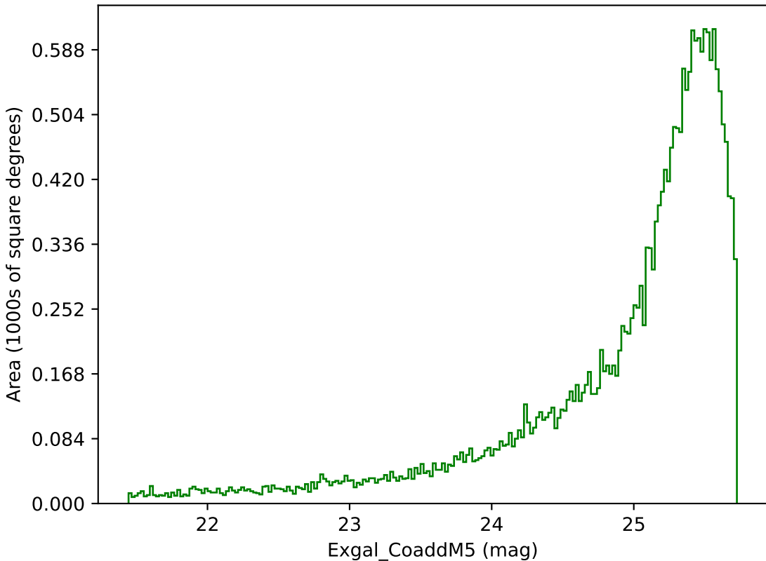
weather_cloudso20v3.4_10yrs Yr 1 g band: Exgal_CoaddM5
