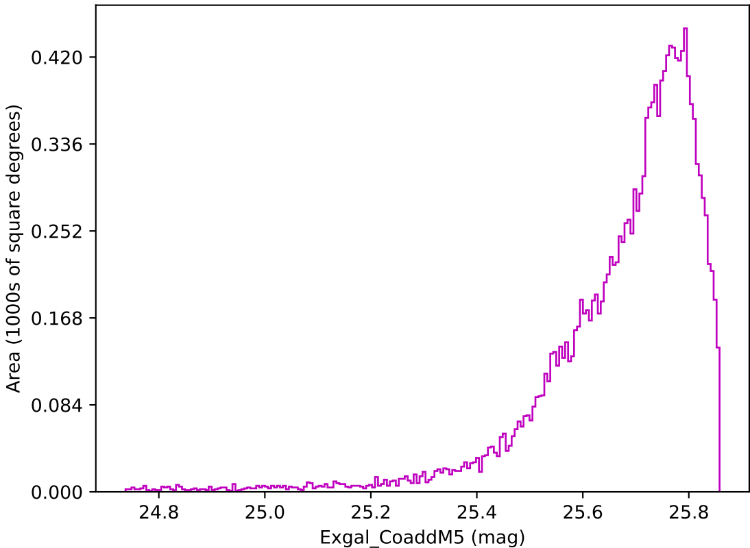
weather_cloudso20v3.4_10yrs WFD z band: Exgal_CoaddM5
