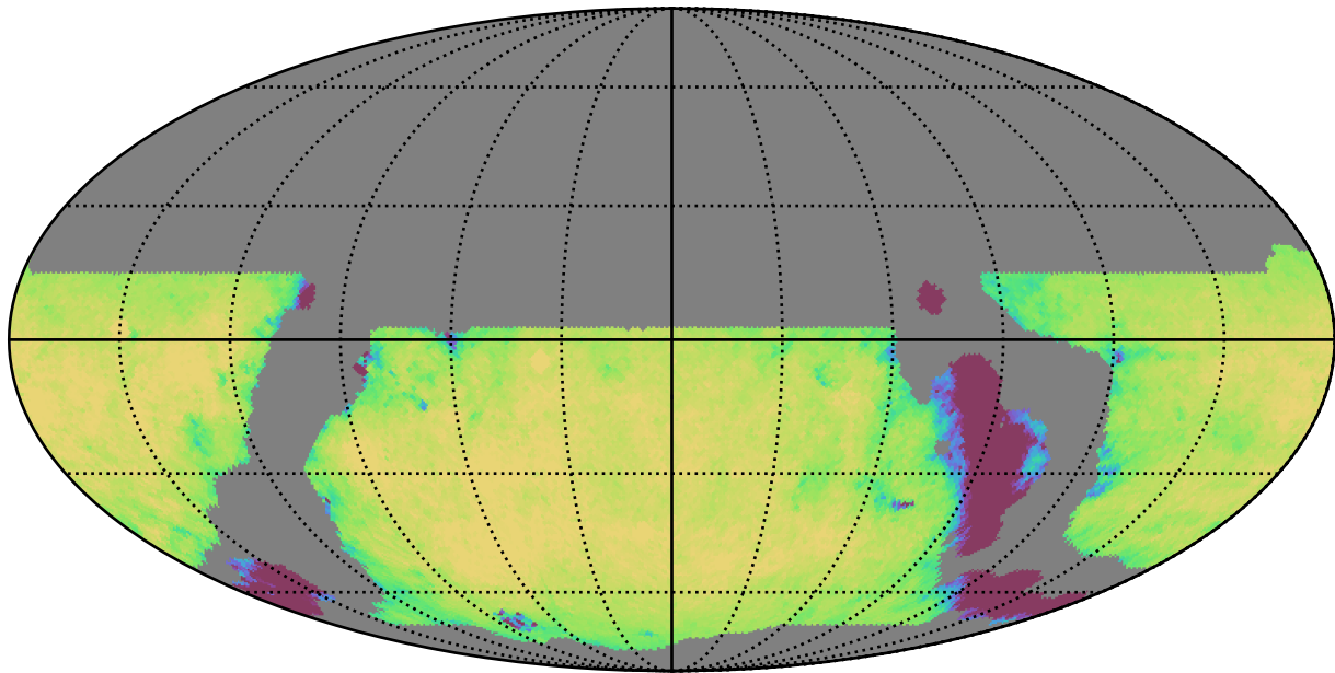
weather_cloudso20v3.4_10yrs WFD u band: Exgal_CoaddM5
