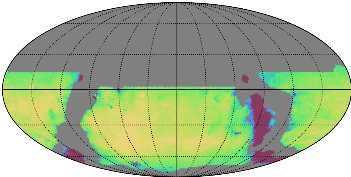
weather_cloudso20v3.4_10yrs WFD r band: Exgal_CoaddM5
