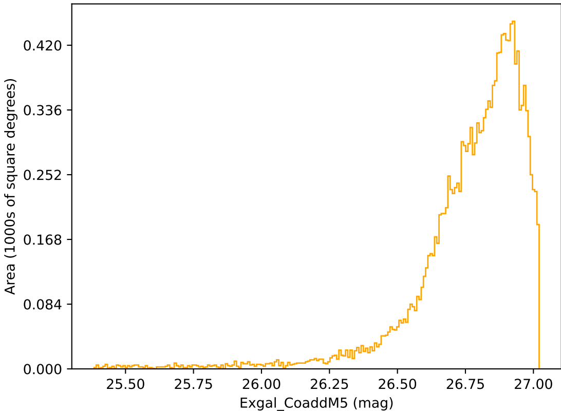
weather_cloudso20v3.4_10yrs WFD r band: Exgal_CoaddM5
