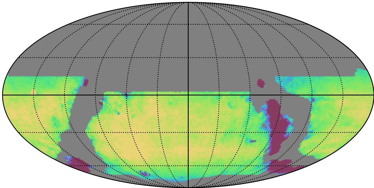
weather_cloudso20v3.4_10yrs WFD i band: Exgal_CoaddM5
