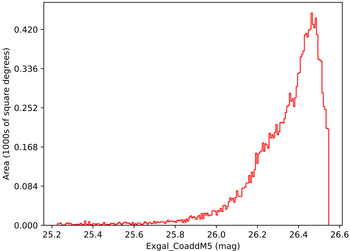
weather_cloudso20v3.4_10yrs WFD i band: Exgal_CoaddM5
