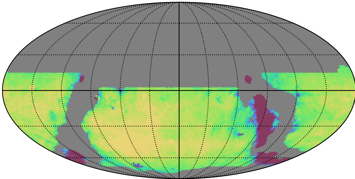
weather_cloudso20v3.4_10yrs WFD g band: Exgal_CoaddM5
