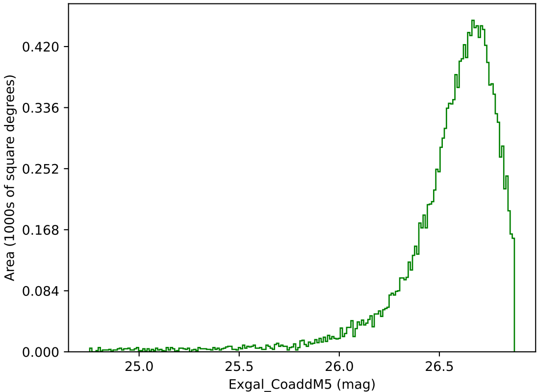
weather_cloudso20v3.4_10yrs WFD g band: Exgal_CoaddM5
