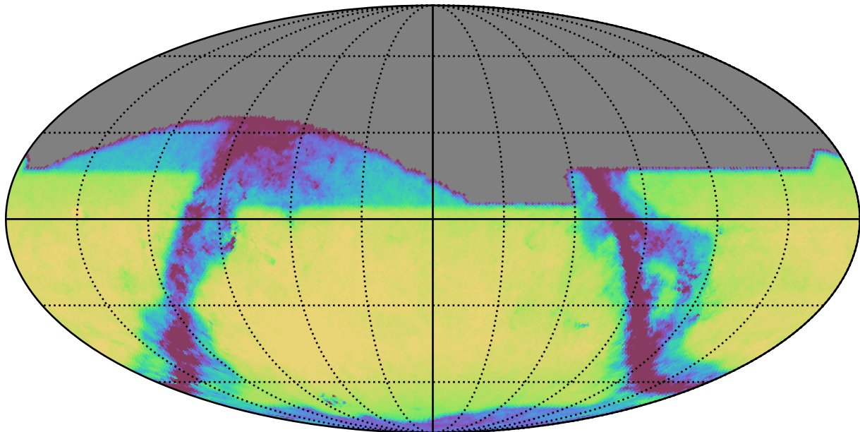
weather_cloudso20v3.4_10yrs All sky z band: Exgal_CoaddM5
