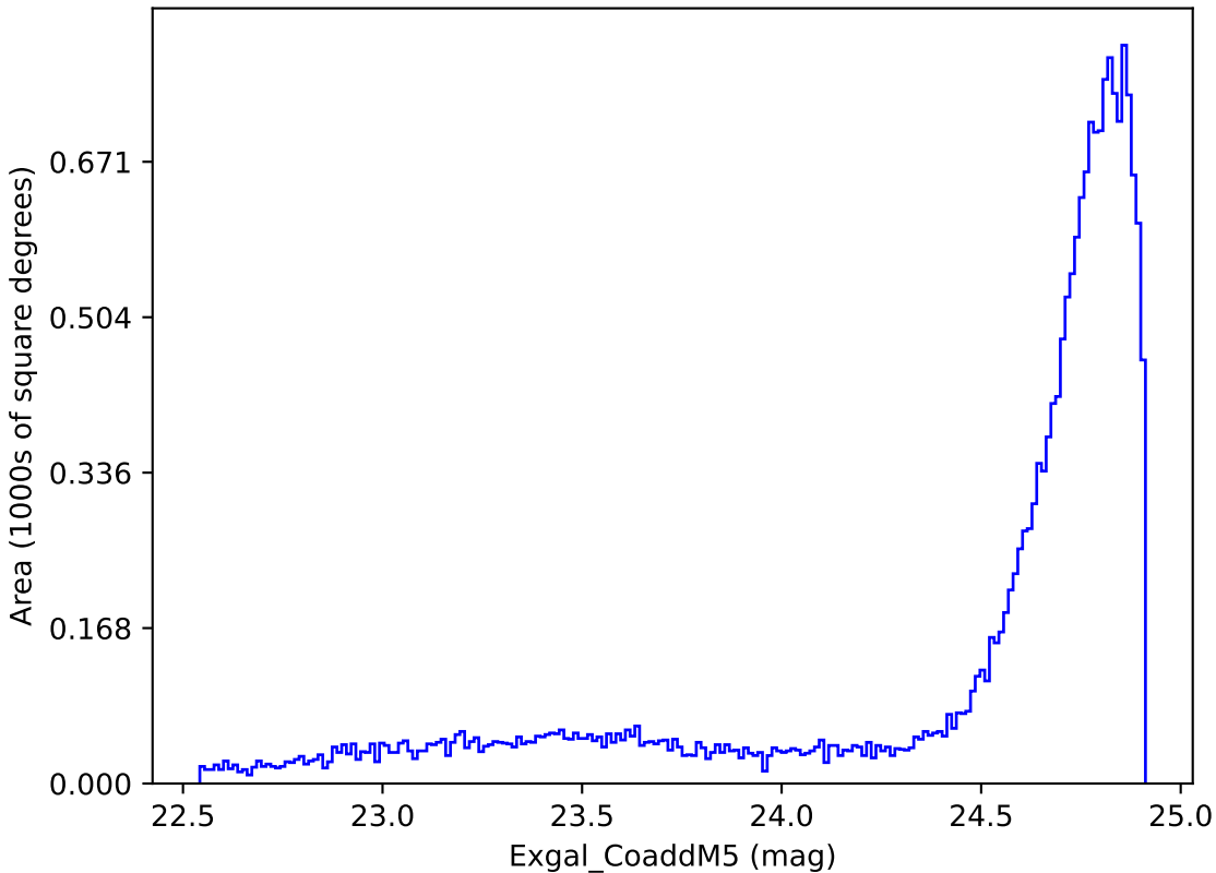
weather_cloudso20v3.4_10yrs All sky y band: Exgal_CoaddM5
