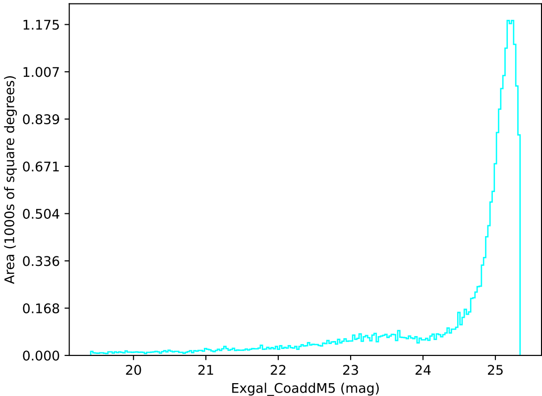
weather_cloudso20v3.4_10yrs All sky u band: Exgal_CoaddM5
