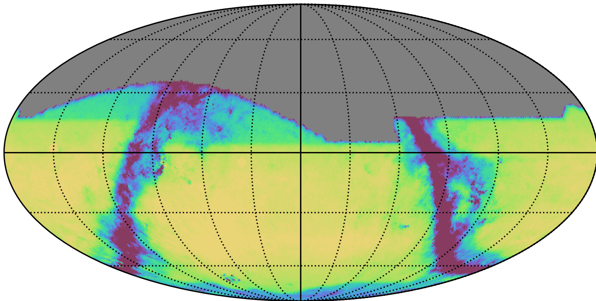
weather_cloudso20v3.4_10yrs All sky r band: Exgal_CoaddM5
