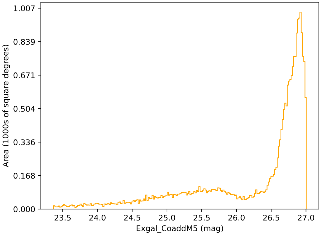
weather_cloudso20v3.4_10yrs All sky r band: Exgal_CoaddM5
