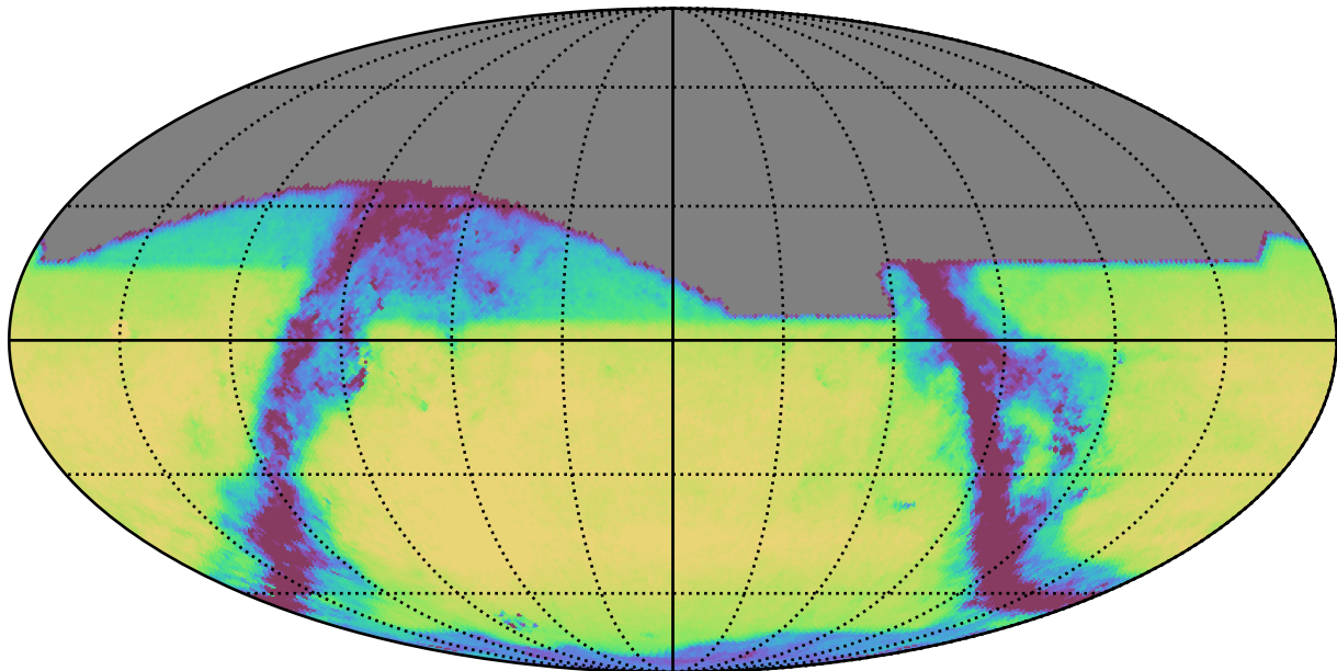
weather_cloudso20v3.4_10yrs All sky i band: Exgal_CoaddM5
