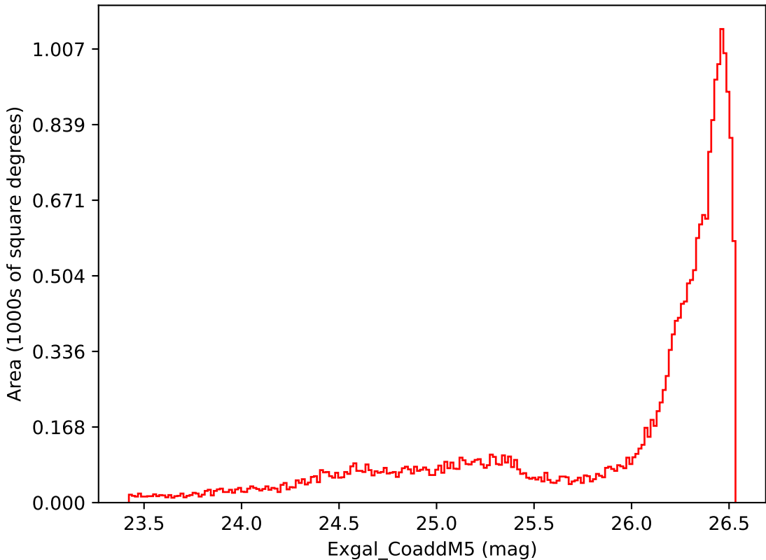
weather_cloudso20v3.4_10yrs All sky i band: Exgal_CoaddM5
