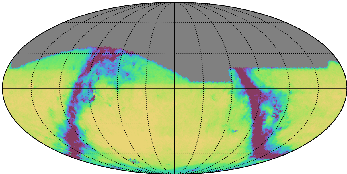
weather_cloudso20v3.4_10yrs All sky g band: Exgal_CoaddM5
