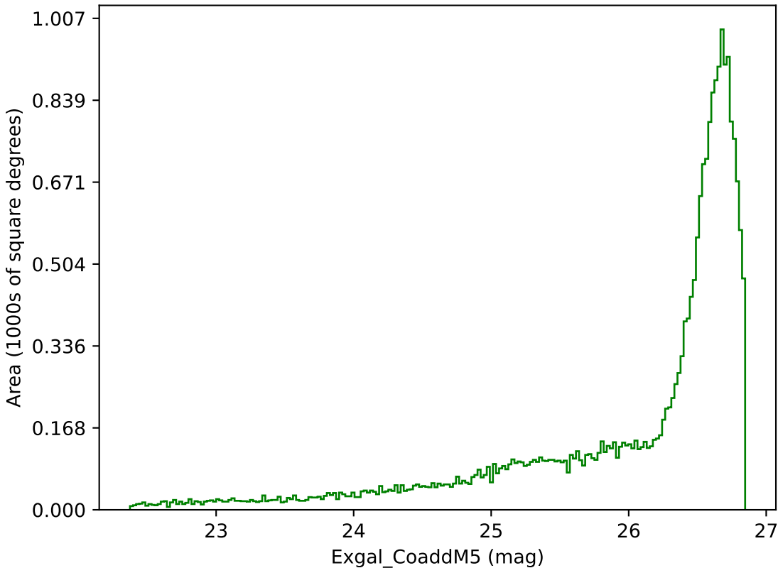
weather_cloudso20v3.4_10yrs All sky g band: Exgal_CoaddM5
