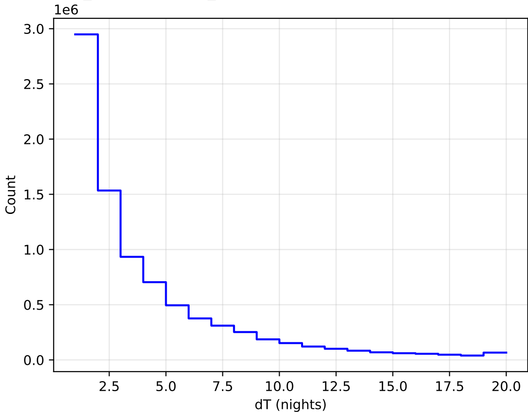
weather_cloudso20v3.4_10yrs WFD all bands: DeltaNight Histogram
