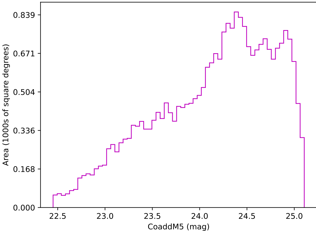
weather_cloudso20v3.4_10yrs Yr 3-4 z band: CoaddM5
