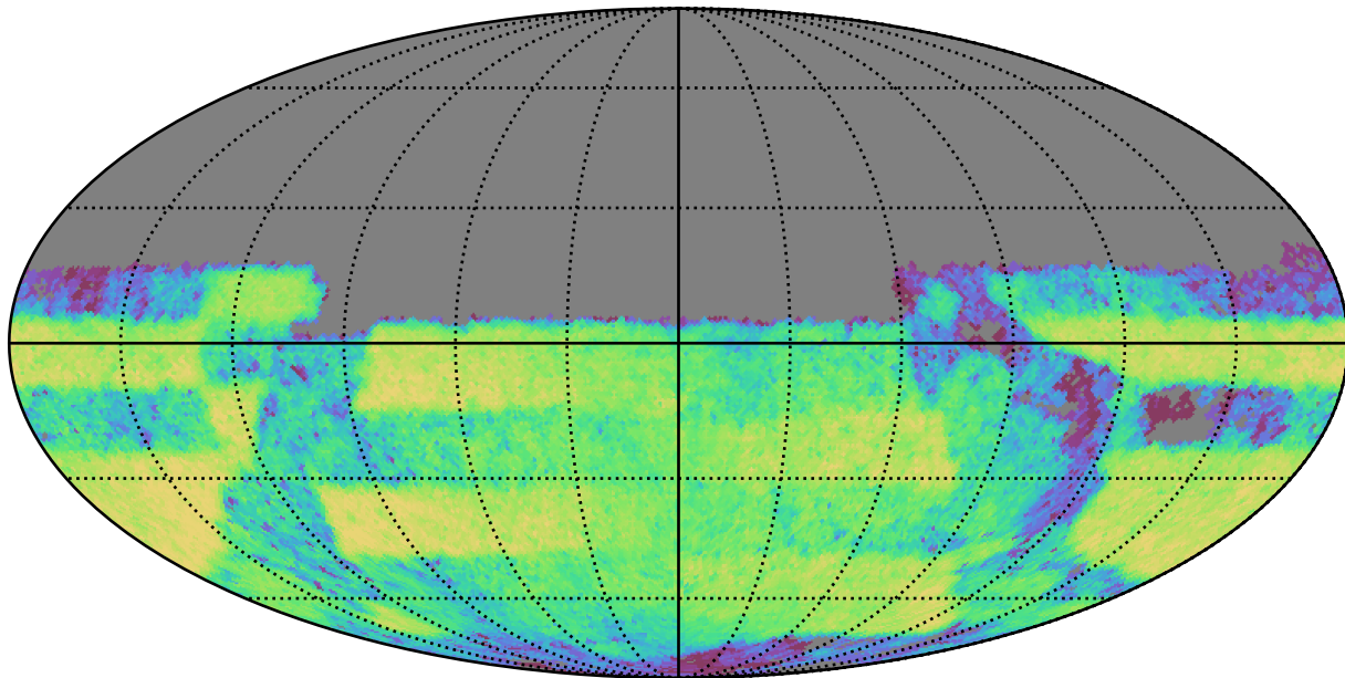
weather_cloudso20v3.4_10yrs Yr 3-4 y band: CoaddM5
