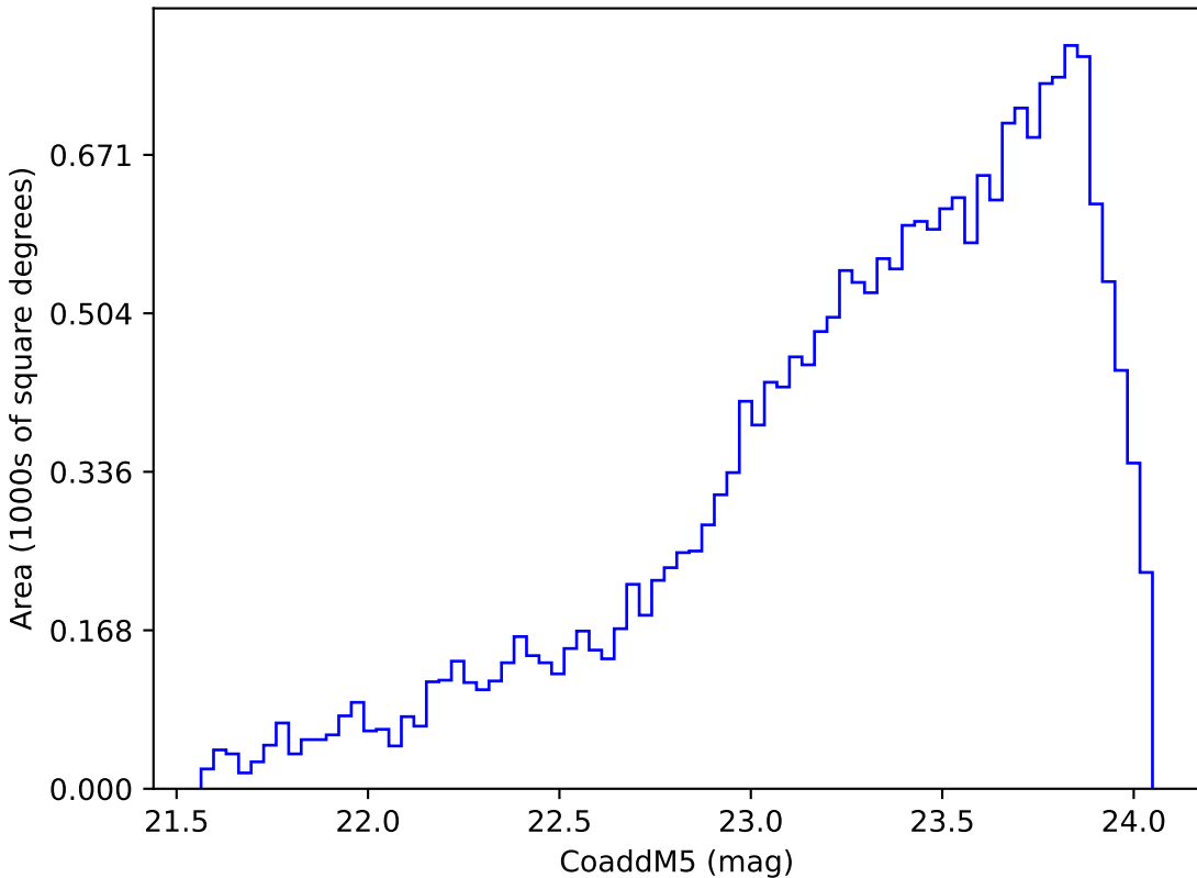
weather_cloudso20v3.4_10yrs Yr 3-4 y band: CoaddM5
