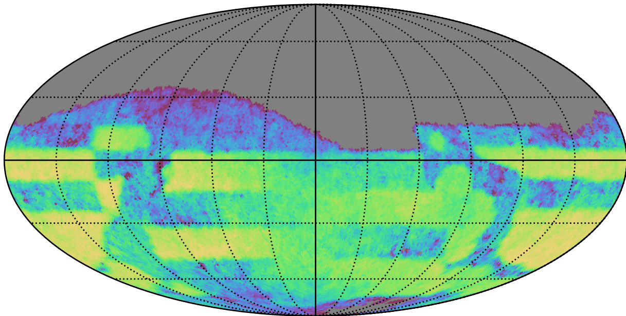
weather_cloudso20v3.4_10yrs Yr 3-4 r band: CoaddM5
