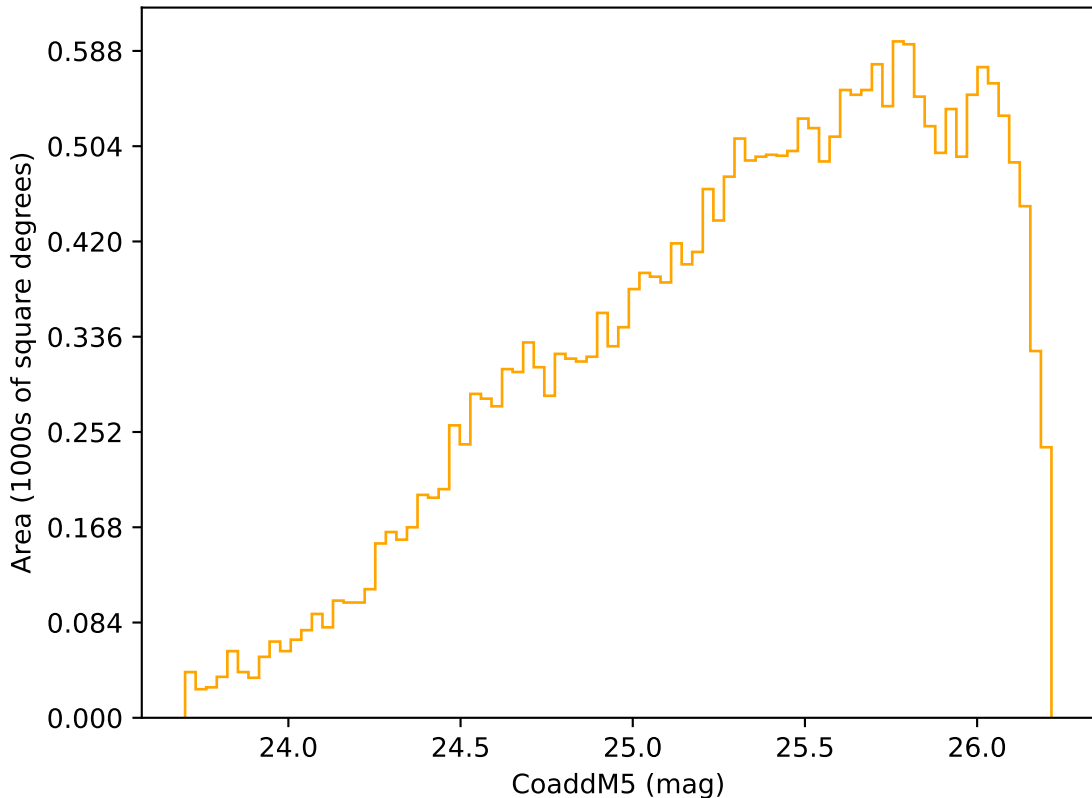
weather_cloudso20v3.4_10yrs Yr 3-4 r band: CoaddM5
