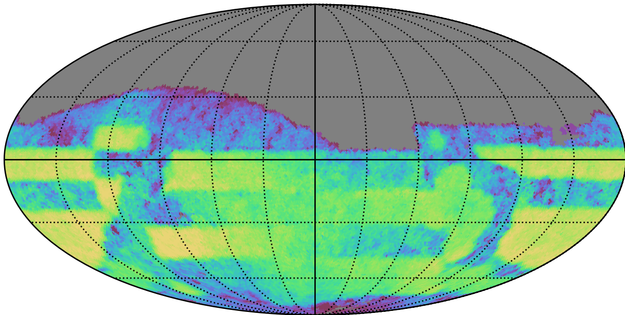
weather_cloudso20v3.4_10yrs Yr 3-4 i band: CoaddM5
