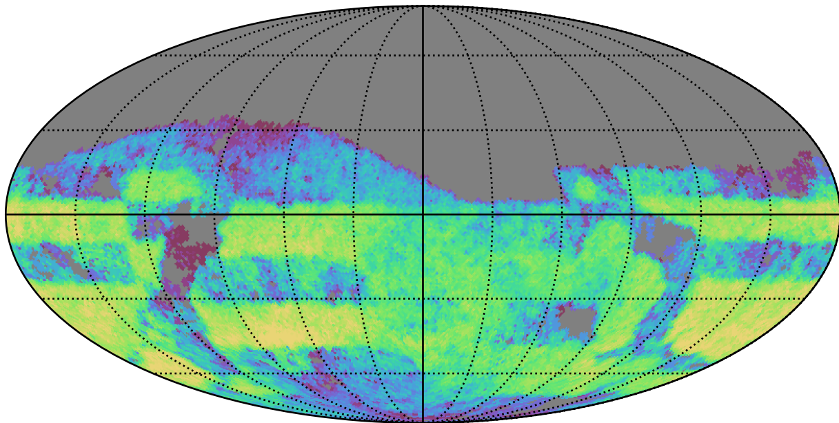
weather_cloudso20v3.4_10yrs Yr 3-4 g band: CoaddM5
