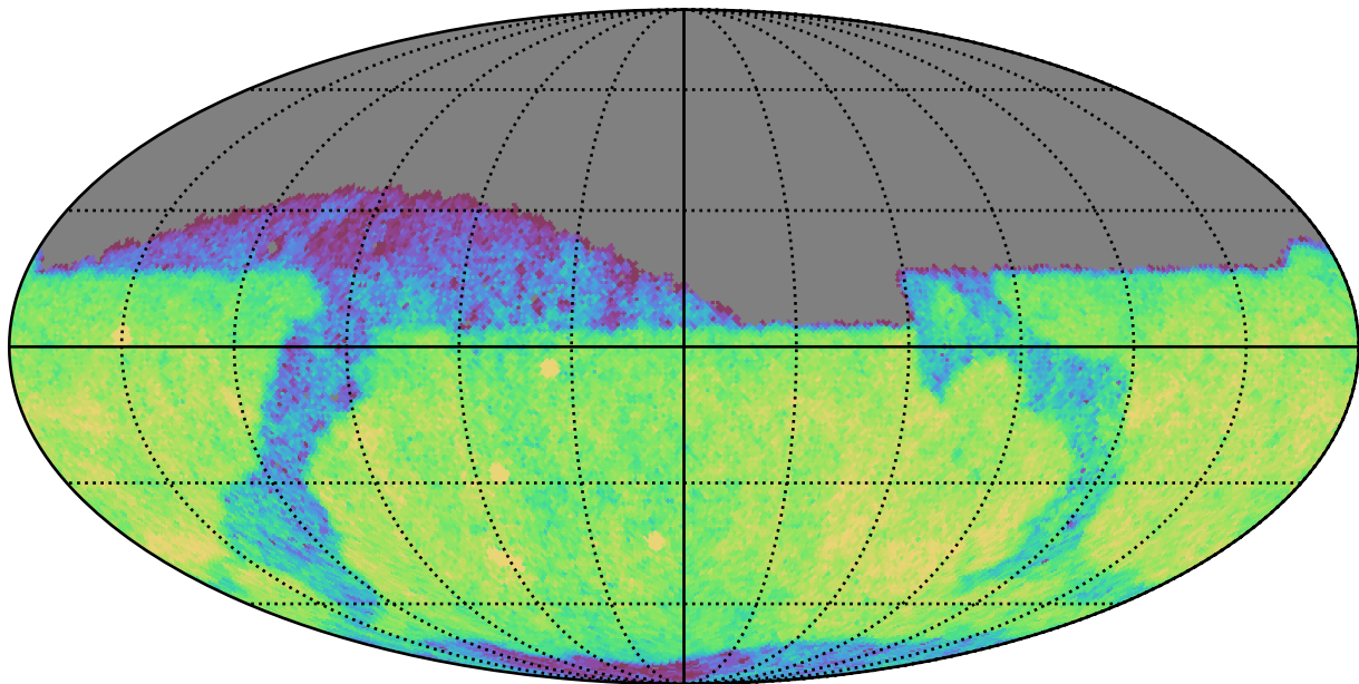
weather_cloudso20v3.4_10yrs Yr 1 z band: CoaddM5
