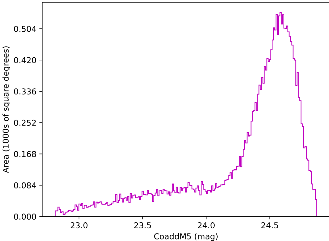
weather_cloudso20v3.4_10yrs Yr 1 z band: CoaddM5
