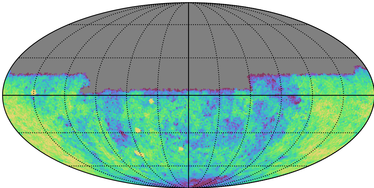
weather_cloudso20v3.4_10yrs Yr 1 u band: CoaddM5
