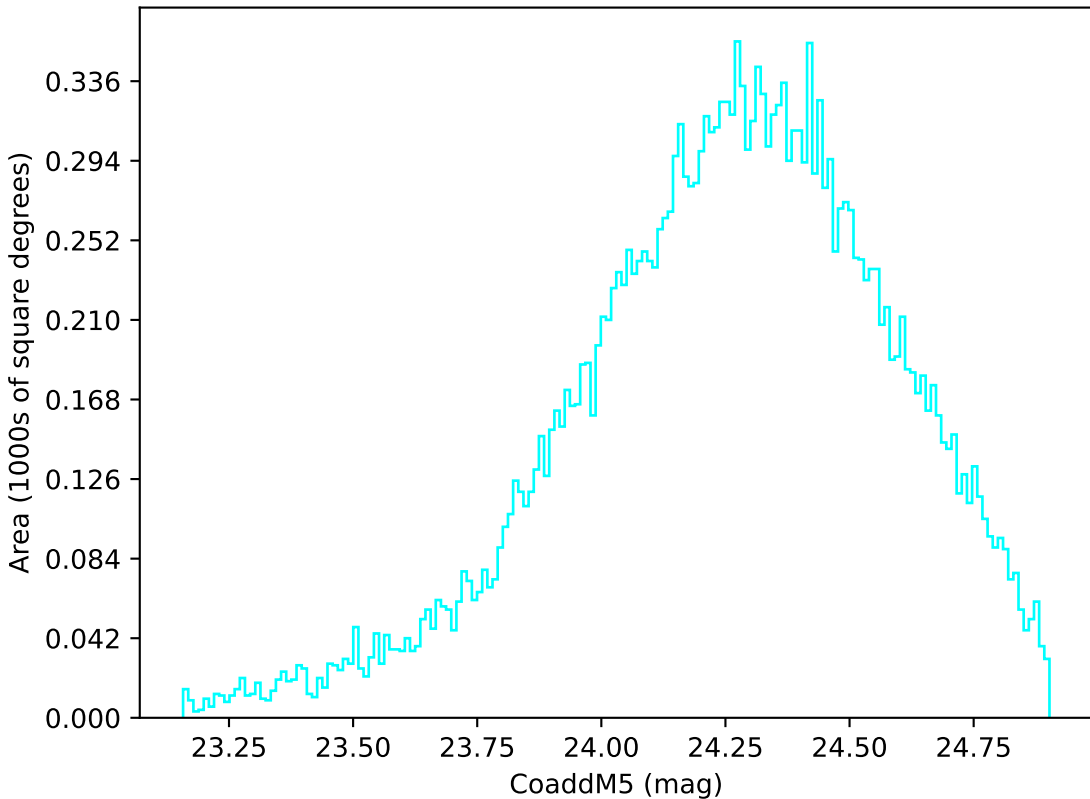
weather_cloudso20v3.4_10yrs Yr 1 u band: CoaddM5
