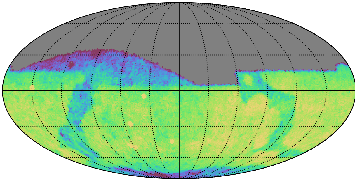
weather_cloudso20v3.4_10yrs Yr 1 r band: CoaddM5
