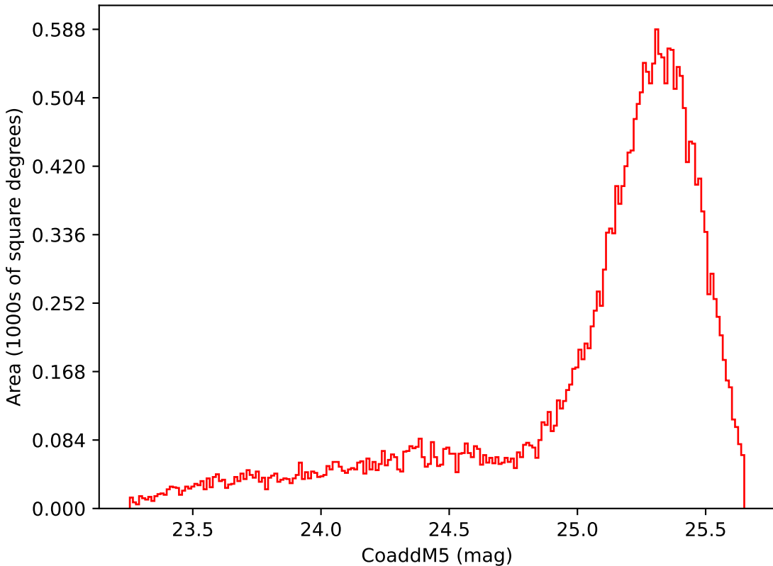
weather_cloudso20v3.4_10yrs Yr 1 i band: CoaddM5
